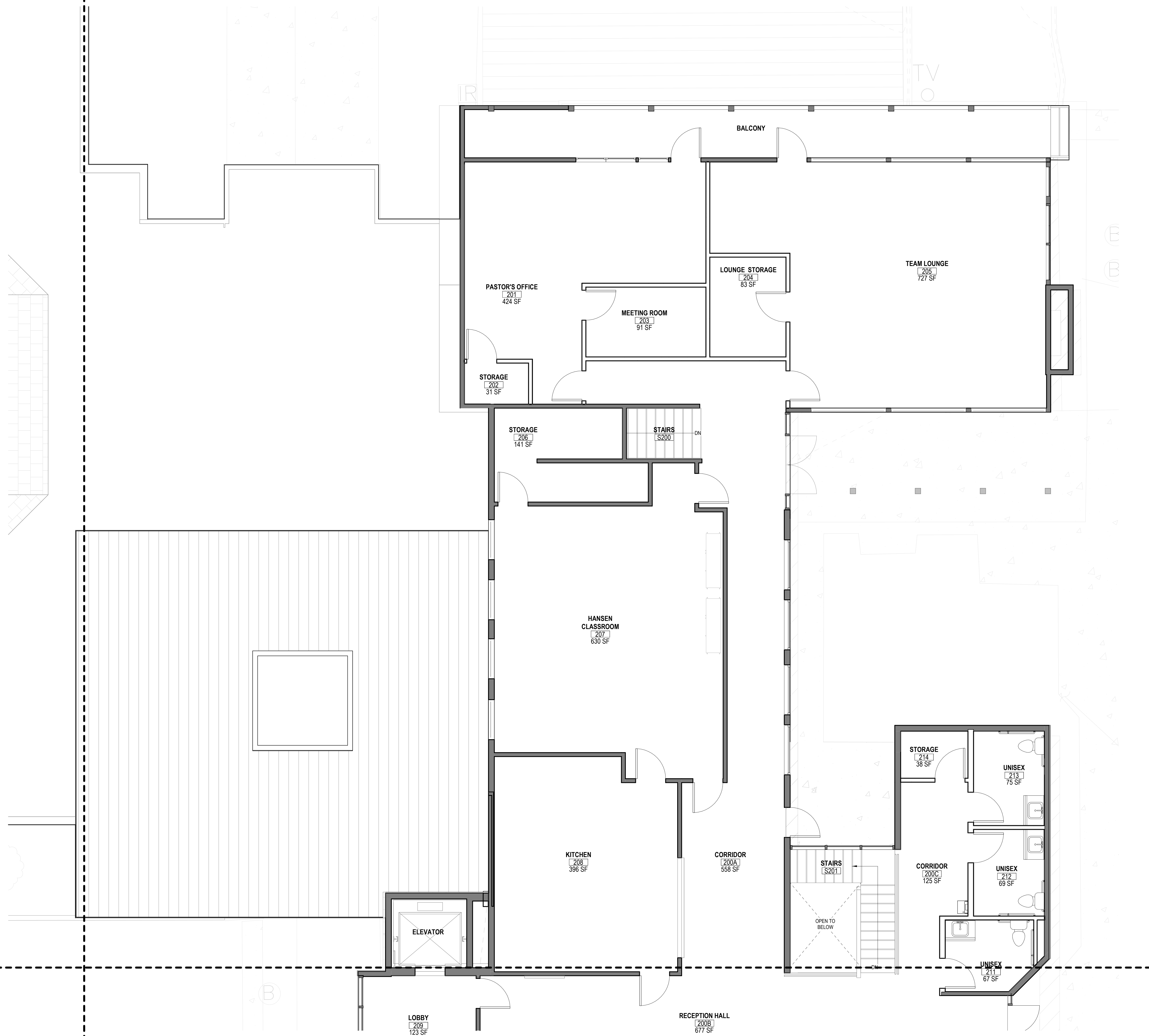
1 LEVEL 2 - NORTHERN MATCHLINE PLAN DR1.02A 1/4" = 1'-0"
