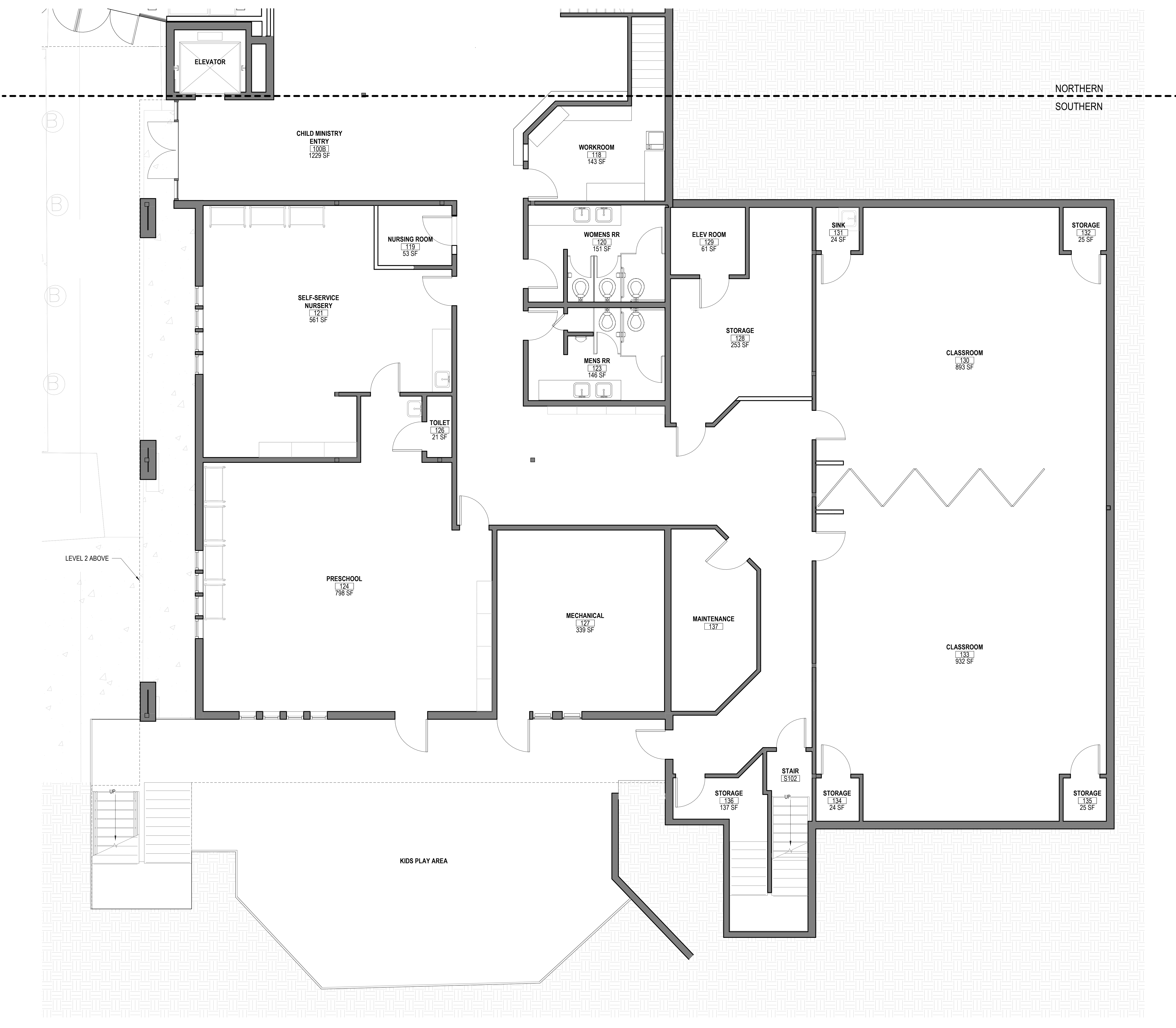
1 LEVEL 1 - SOUTHERN MATCHLINE PLAN DR1.01C 1/4" = 1'-0"
