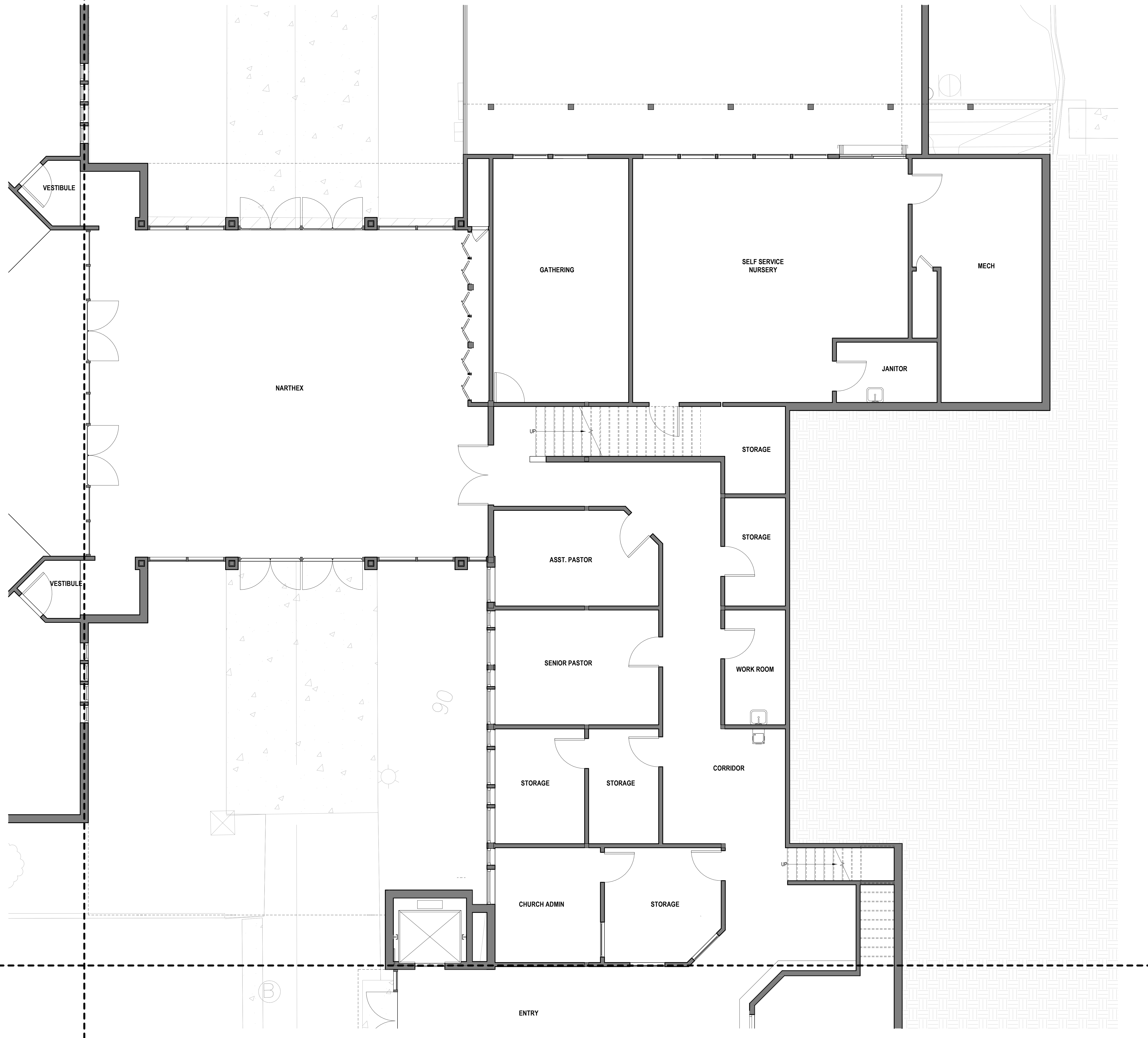
1 LEVEL 1 - NORTHERN MATCHLINE PLAN EX1.01B 1/4" = 1'-0"
